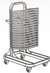
ROUND / SQUARE TOP TRANSFER AND STORAGE CART L40" W31" H61" L101cm W79cm H155cm holds up to 16 CliX round/square tops
