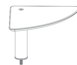
LARGE TRIANGLE HIGH DISPLAY SHELF L17" W17" H12.5" L44cm W44cm H32cm
